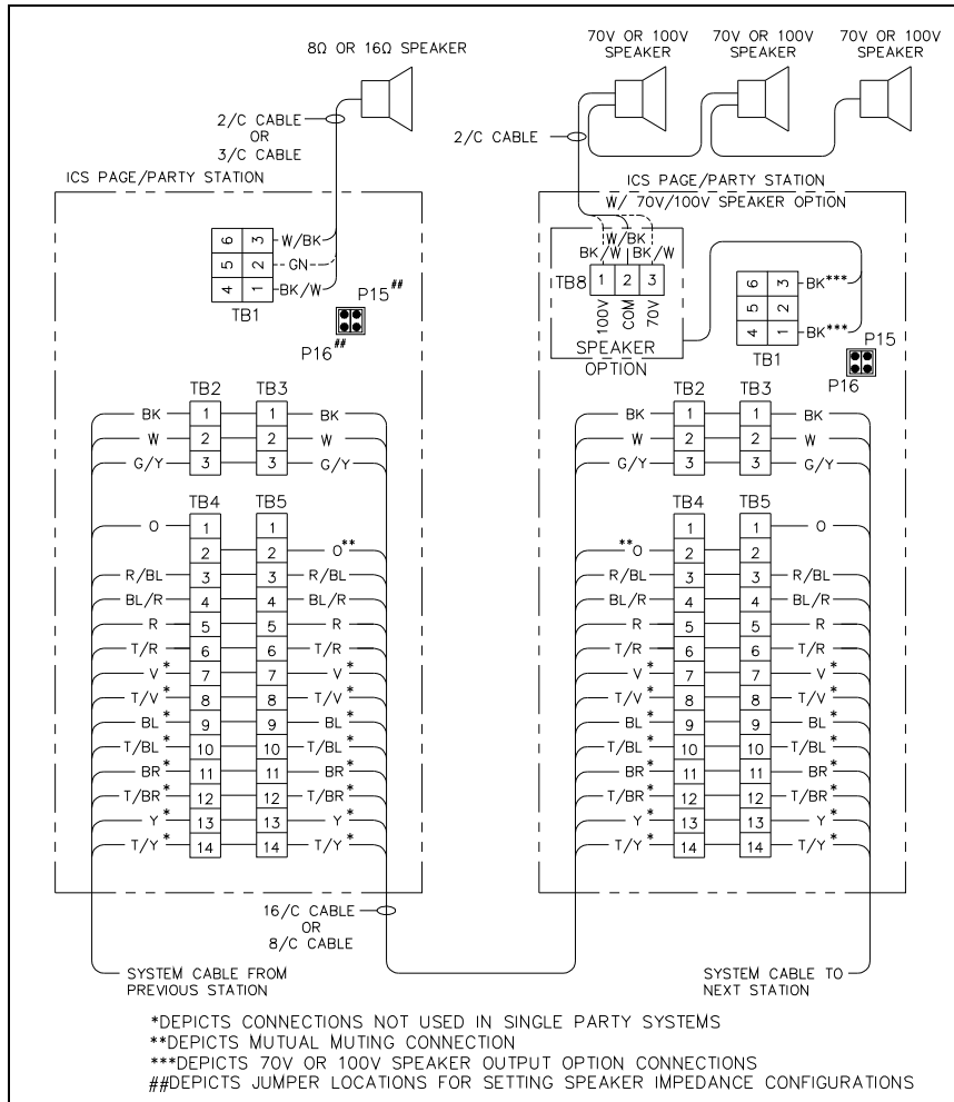
Figure 3. Typical installation wiring configuration
