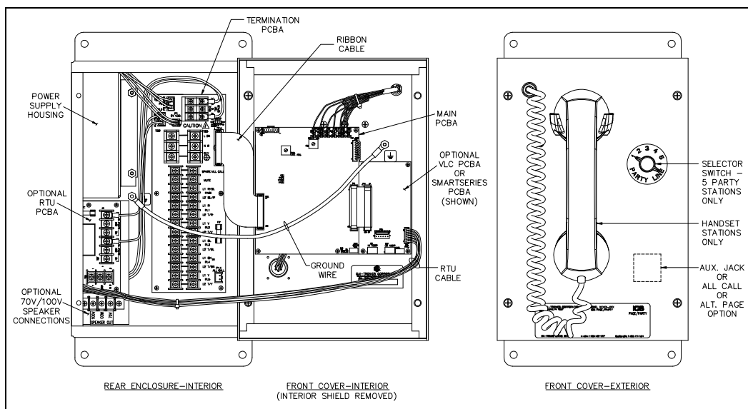
Figure 1. ICS Station with available options (AC Version shown)
